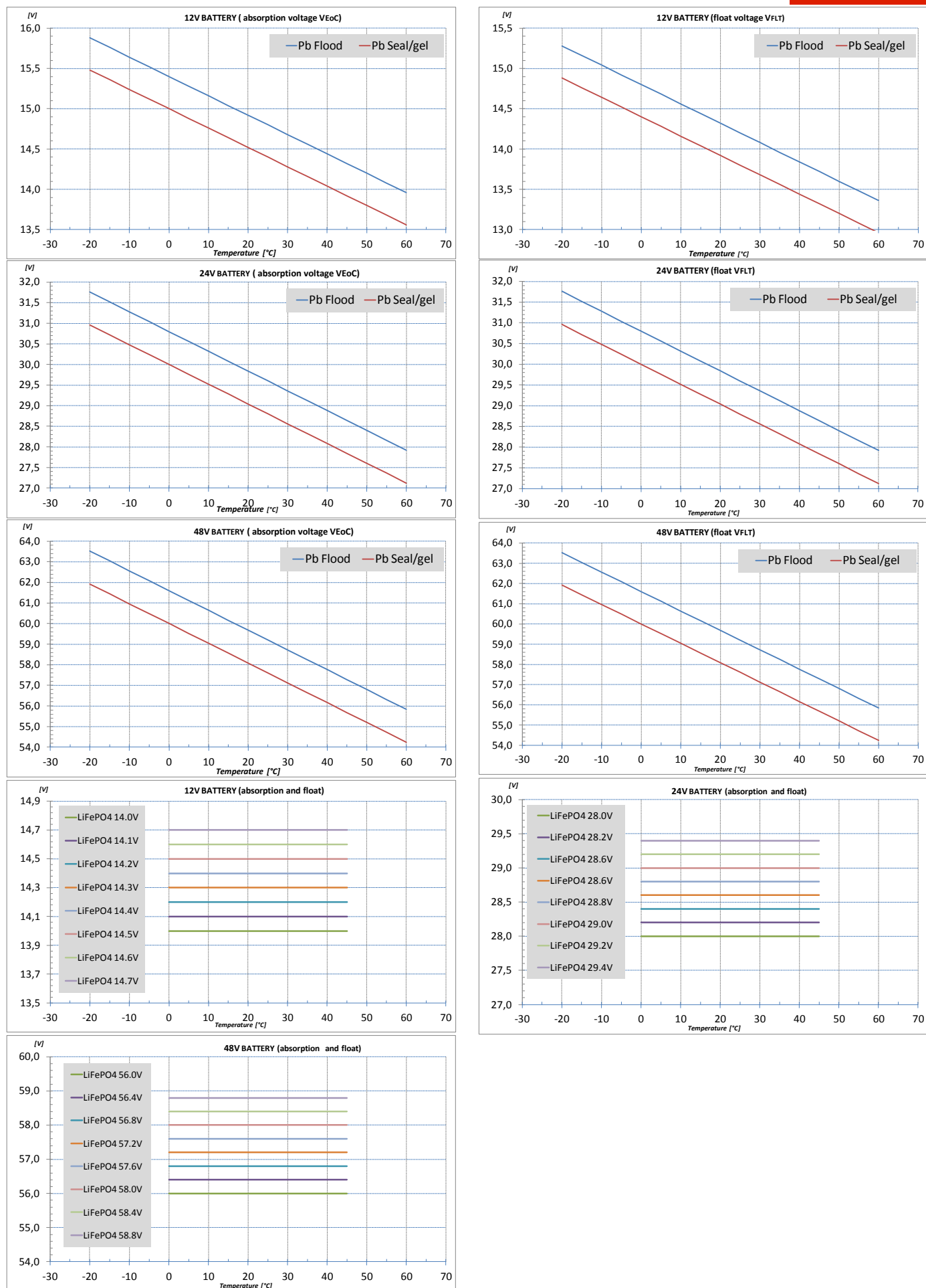
Pic.5 - Absorption voltage and float voltage as a function of temperature
