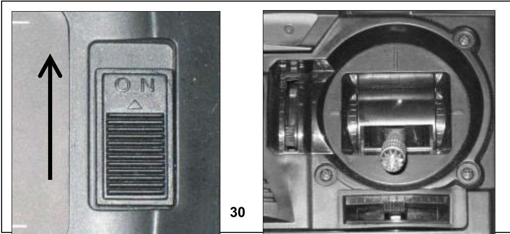
Fig. 30 - Switch the transmitter on and move the throttle stick to the "OFF" position (Diagram shows right joystick as throttle control stick which is on MODE 1).
