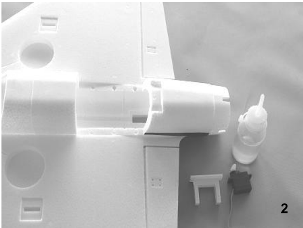
Fig. 2 - Locate the servo fix base and rudder servo
