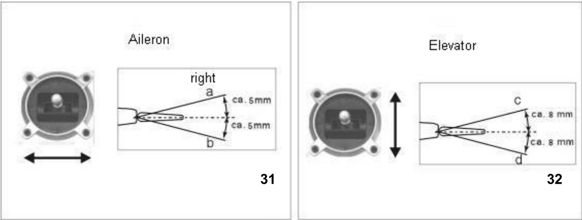
Fig. 31 and 32 - Checking Ailerons and Elevators
