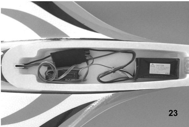
Fig. 23 - Connect the electronic speed controller and servos to the receiver. Refer to the radio instructions for the correct channel sockets and servo lead polarity. Position the battery. Charge the battery according to the safety instructions before installing.
