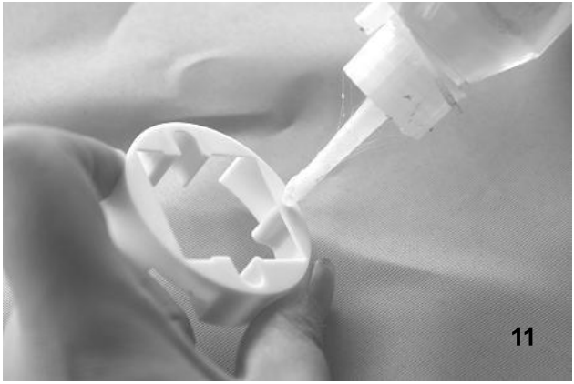
Fig. 11 - Apply glue to the sides of the servo fairing
