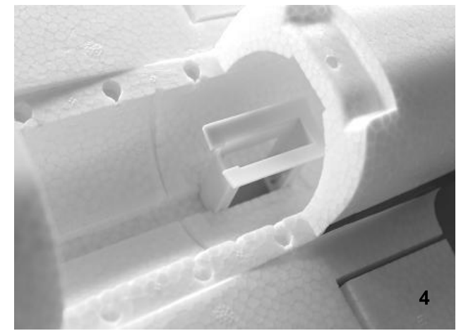
Fig. 4 - Assemble the plastic part into fuselage.
