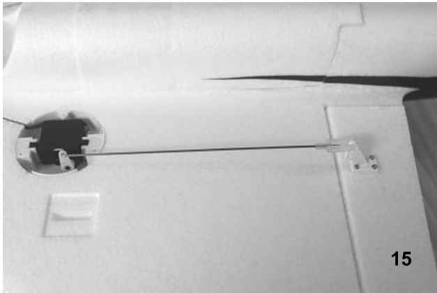
Fig. 15 - Connect the push rods to the servo arm and then to the control horn.
