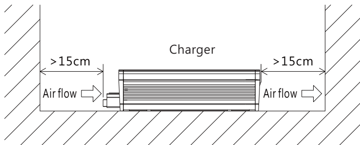
Figure 3-1 set-up recommendation
