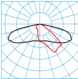
LIQ 50N-AB2L-LRA/1800-722 2G1 ETDD (CLO initial value) TX280886 ■ C0 - C180 ■ C90 - C270 DIN 5040: A30 UTE: 1,00 G CEN Flux Code: 34 71 96 100 100 0 0 0 0
