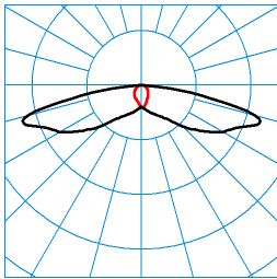
LIQ 50N-SB3L-LR-SLR2/2200-740 2G1 ET (CLO initial value) TX278161 ■ C0 - C180 ■ C90 - C270 DIN 5040: A30 UTE: 1,00 l CEN Flux Code: 31 64 92 100 100
