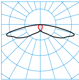
LIQ 50N-SB3L-LR-SLR2/2200-740 2G1 ET (CLO end value) TX277673 ■ C0 - C180 ■ C90 - C270 DIN 5040: A30 UTE: 1,00 l CEN Flux Code: 31 64 92 100 100
