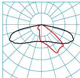
LIQ 50N-AB2L-SLR1/6800-722 6G1 ET (CLO initial value) TX280922 ■ C0 - C180 ■ C90 - C270 DIN 5040: A30 UTE: 1,00 G CEN Flux Code: 34 71 96 100 100 0 0 0 0
