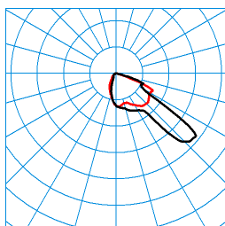
LIQ 70N-FR1L/6800-727 8G1 ET(CLO initial value) TX278341 ■ C0 - C180 ■ C90 - C270 DIN 5040: A40 UTE: 1,00 F CEN Flux Code: 41 83 99 100 100
