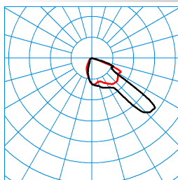
LIQ 70N-FR1L/6800-727 8G1 ET(CLO end value) TX278168 ■ C0 - C180 ■ C90 - C270 DIN 5040: A40 UTE: 1,00 F CEN Flux Code: 41 83 99 100 100
