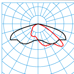
LIQ 70N-AB7L-LRA/8200-722 10G1 ETDD (CLO end value) TX281079 ■ C0 - C180 ■ C90 - C270 DIN 5040: A30 UTE: 1,00 G CEN Flux Code: 35 73 98 100 100 0 0 0 0
