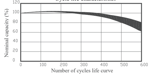
Cycle life characteristics
