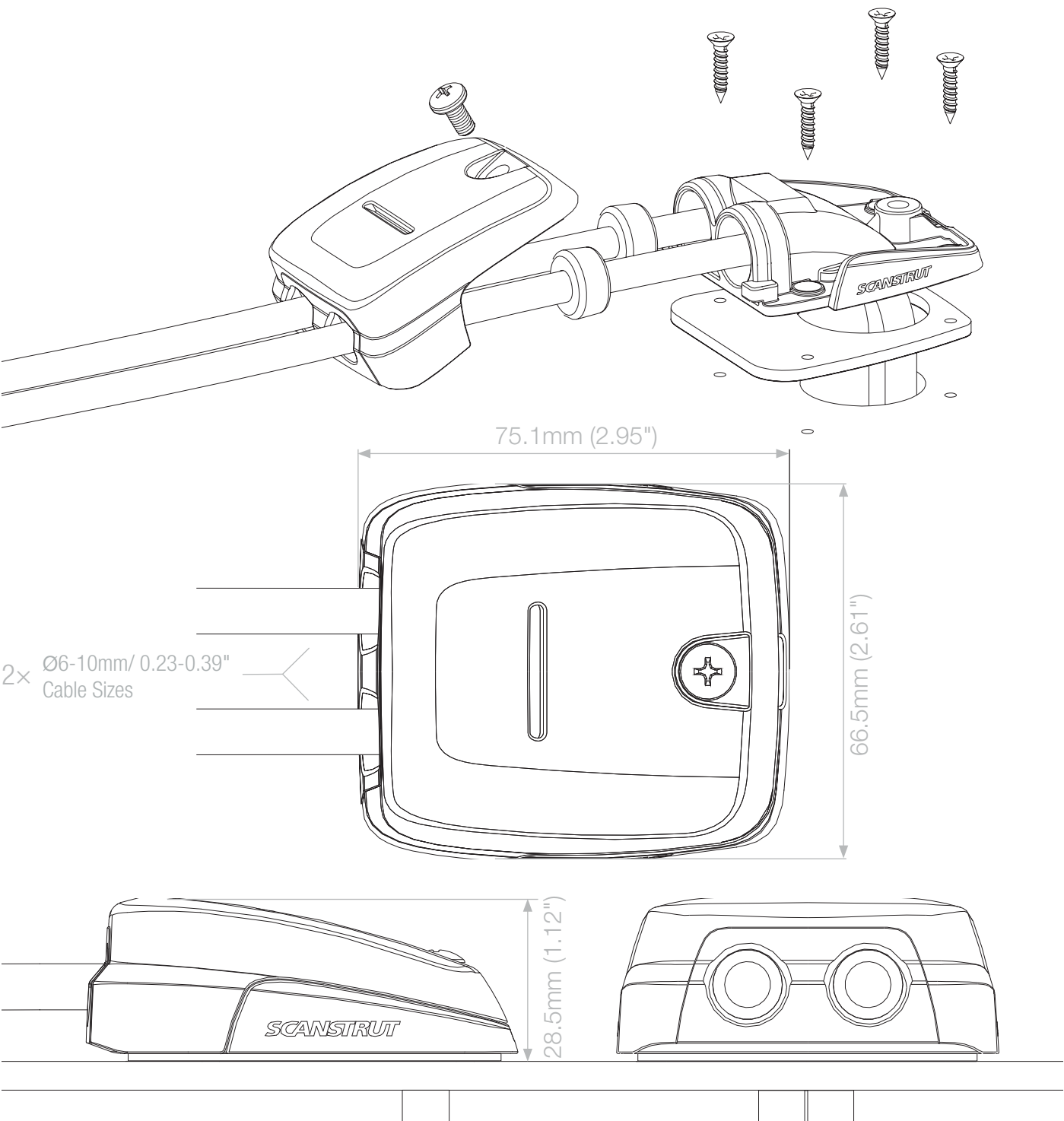
Bung dimensions for different models (included in the package)
