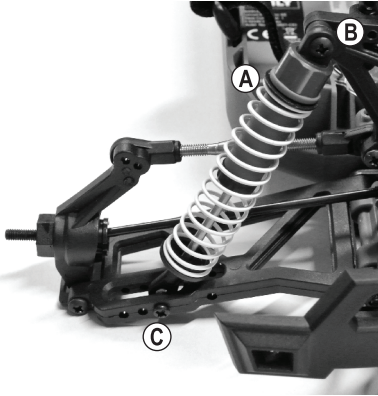
Front axle
