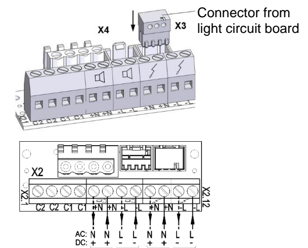
Operating voltage connection for sounder
