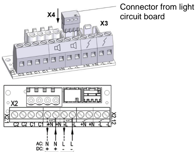
Operating voltage connection
