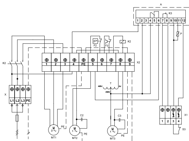
NSYCU..2K3P4 – NSYCU..2K3P4..
