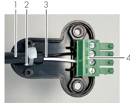
Figure 4 PT1000 adapter
