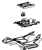
500801028 Karosserie Body KOD Pickup GP
