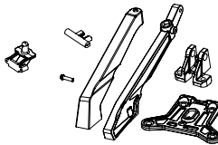
500405920 Chassis-Streben / Kar.-Halter vo/hi Chassis brace set / Body-mount
