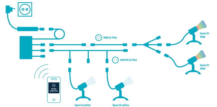
Example 2: WHITE and RGB spotlights in one system (controller required)
