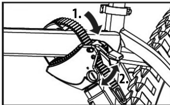
Figure 11: Fastening the bicycle with tension straps
