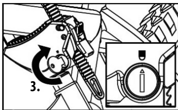
Figure 12: Locking the frame holder
