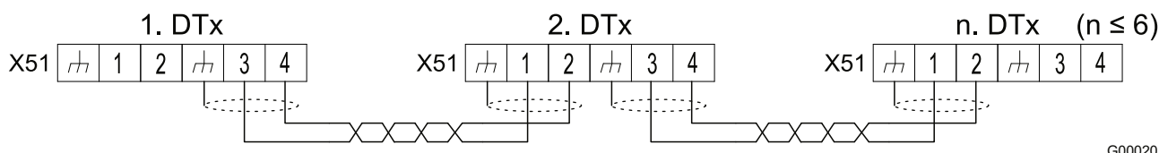
Fig. 23: Controllo Multimaster
