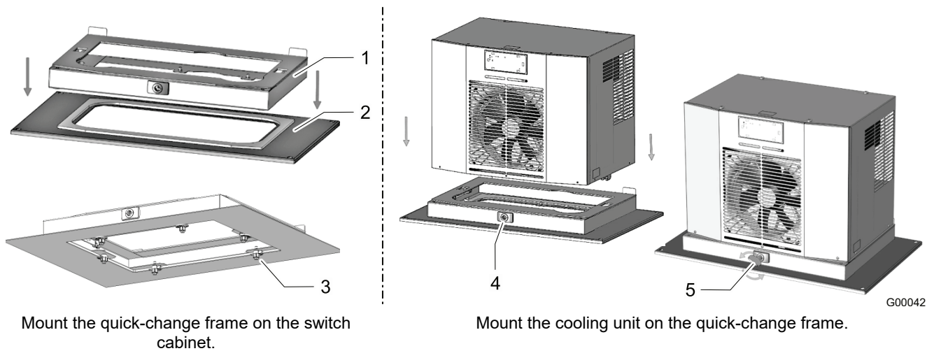
Fig. 21: Mounting the bracket
