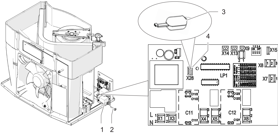
Fig. 28: Service interface
