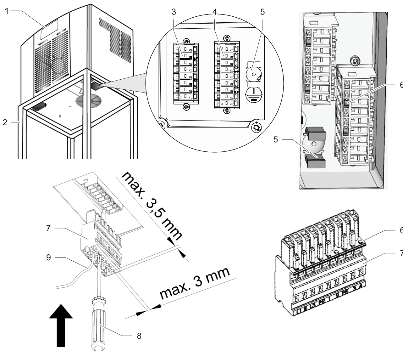
Fig. 25: Cooling unit mains plug
