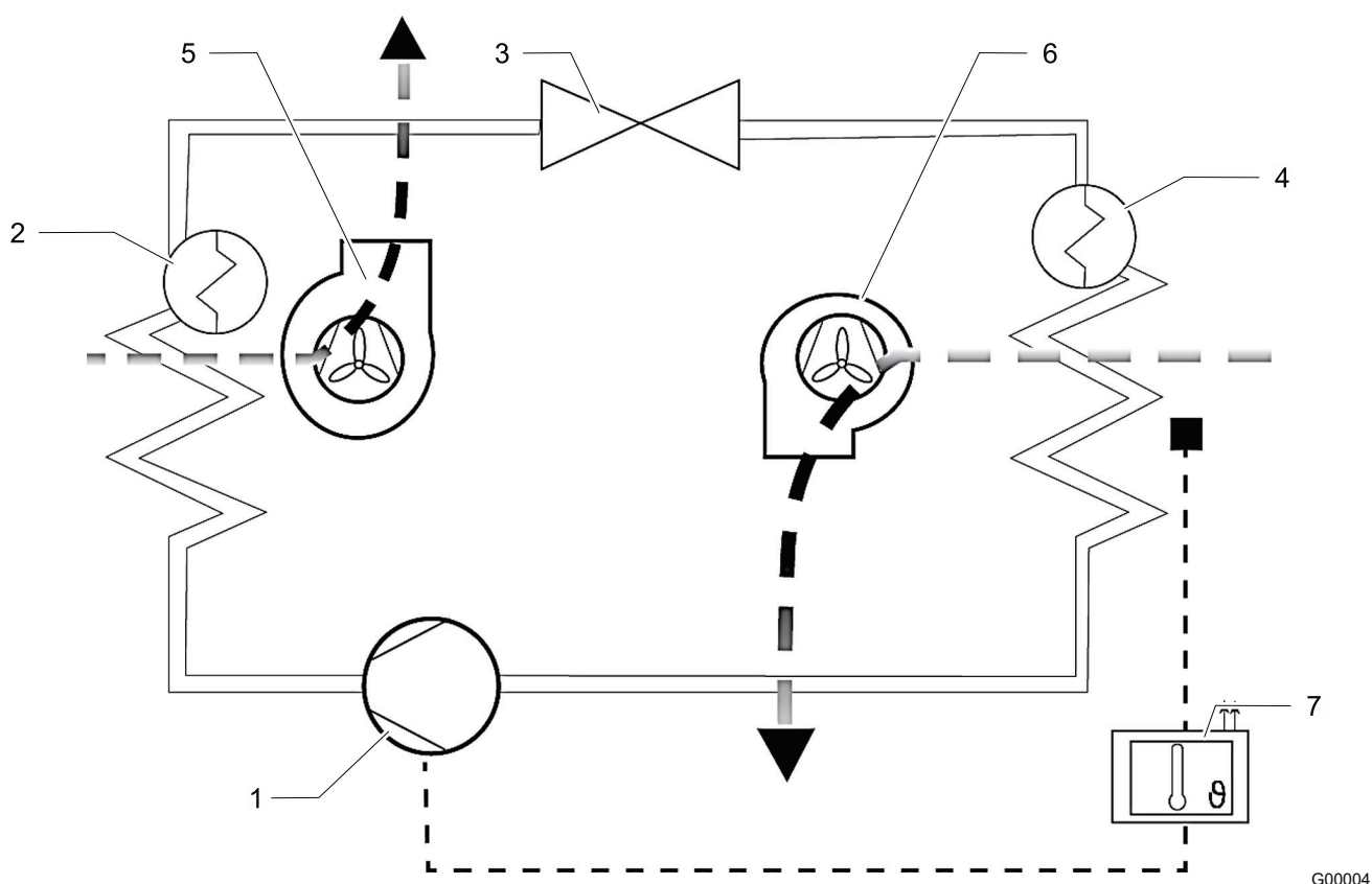
Fig. 7: circuit frigorifique
