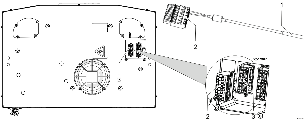
Fig. 24: Temperature sensor - TS2
