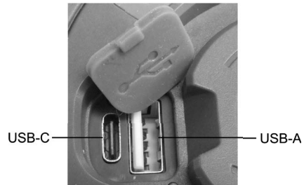
Fig. 2: USB ports
