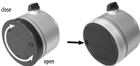
Image 2: opening the battery compartment
