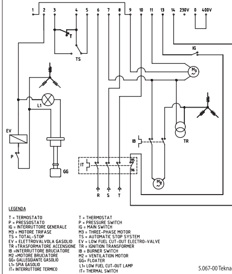
XP_3Ph
