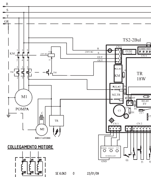
LP_3Ph_220V
