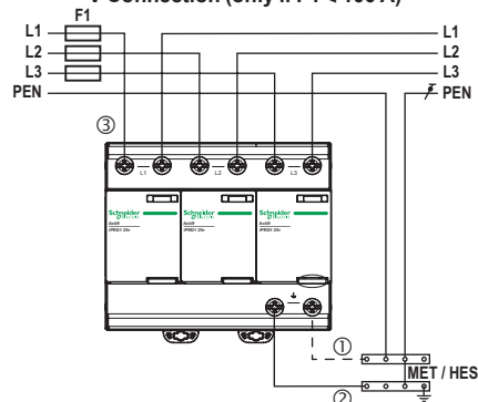
TN-C System, 3+0 V Connection (only if F1 ≤ 100 A)
