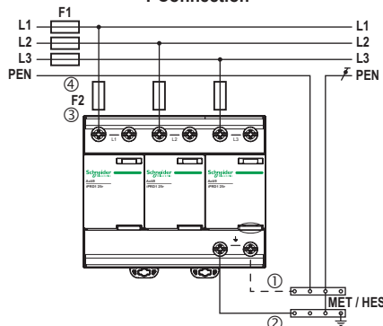
TN-C System, 3+0 T Connection
