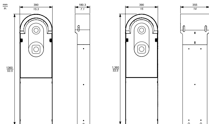
FS1CP: floor standing 1 charge point EVA1RFSK1
