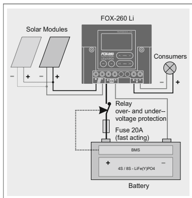
Diagram: 1-Channel Protection
