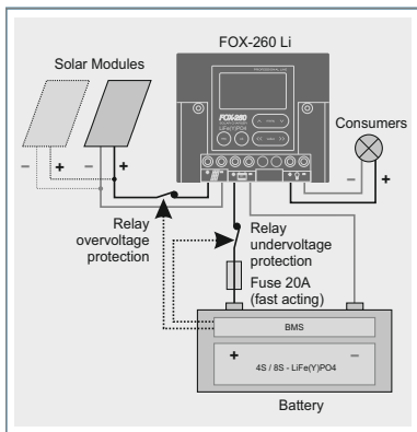
Diagram: 2-Chanel Protection
