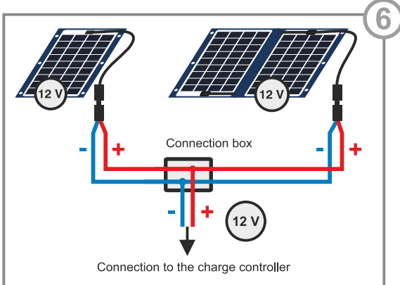
Picture 6: Parallel connection of the solar modules
