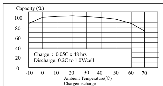
Charging Efficiency
