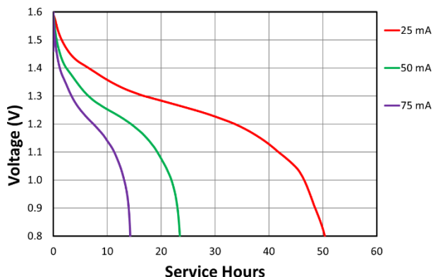
Constant Current
