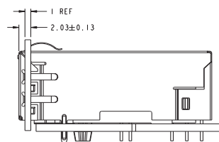
CONNECTOR ASSEMBLED TO PANEL AND PCB
