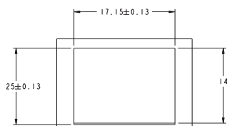
SUGGESTED PANEL CUTOUT
