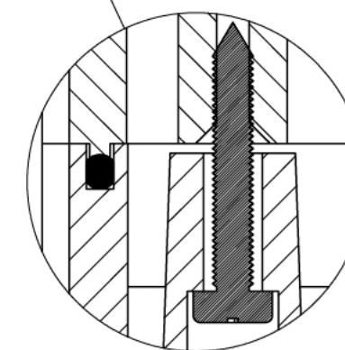
Detalle/Detail/T Escala/Scale 2 : 1
