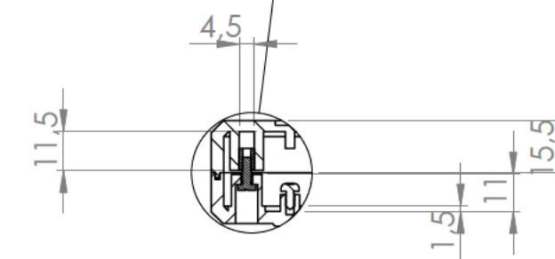
Detalle/Detail R
