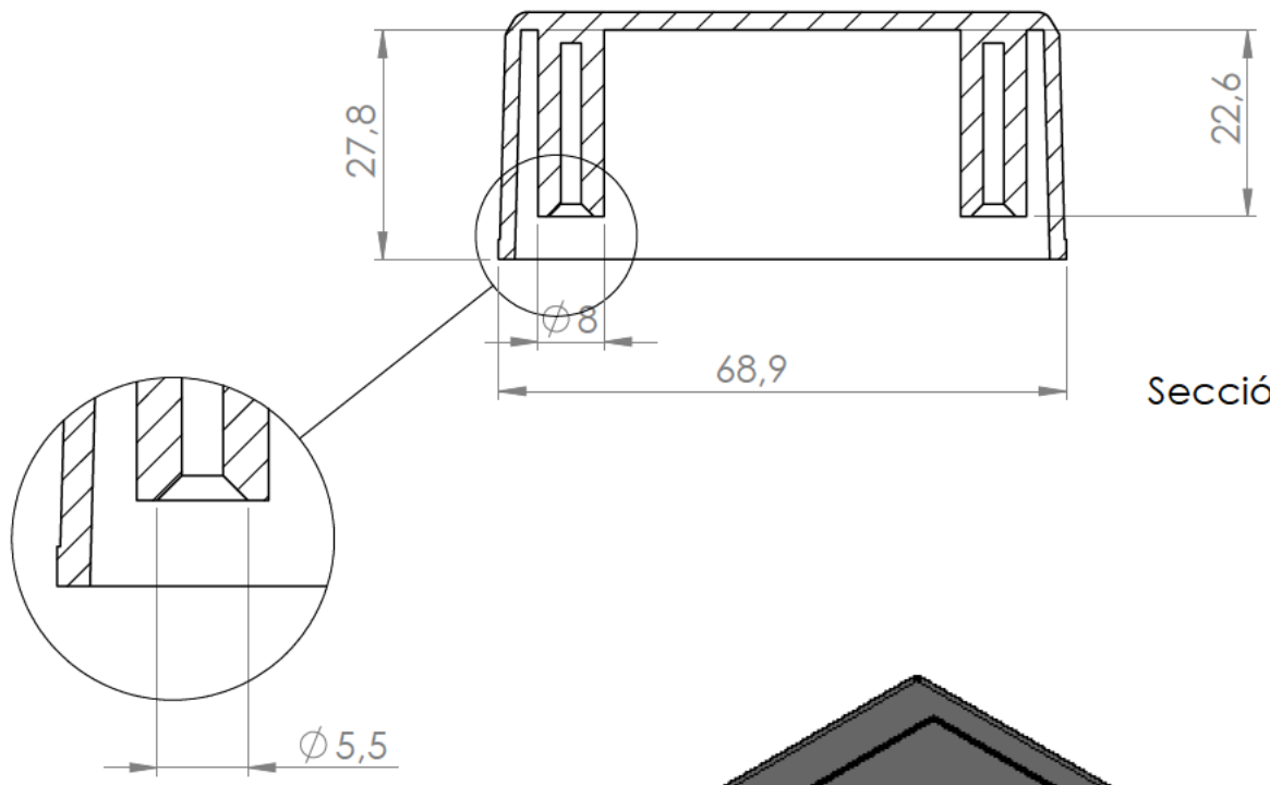
Detalle/Detail P Escala/Scale 2 : 1
