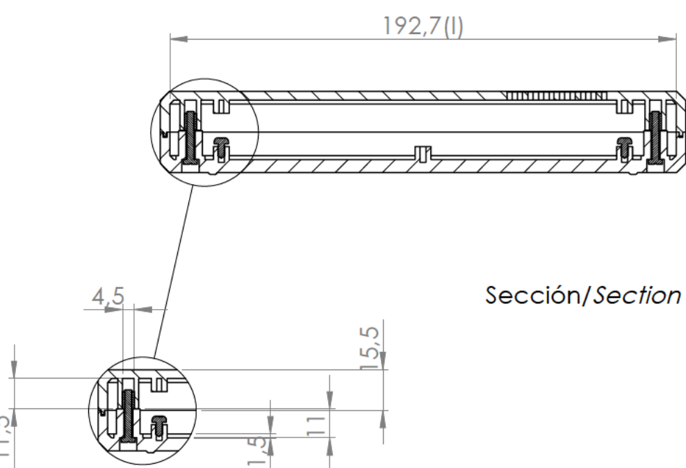
Detalle/Detail R
