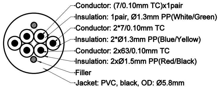
Cable Structure
