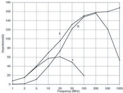
Z-f Characteristics
