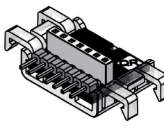
Fig.: Output bus connector for the 800-CON transfer module (1 HP; see Technical data) at the output of a series of measurement devices and modules.
