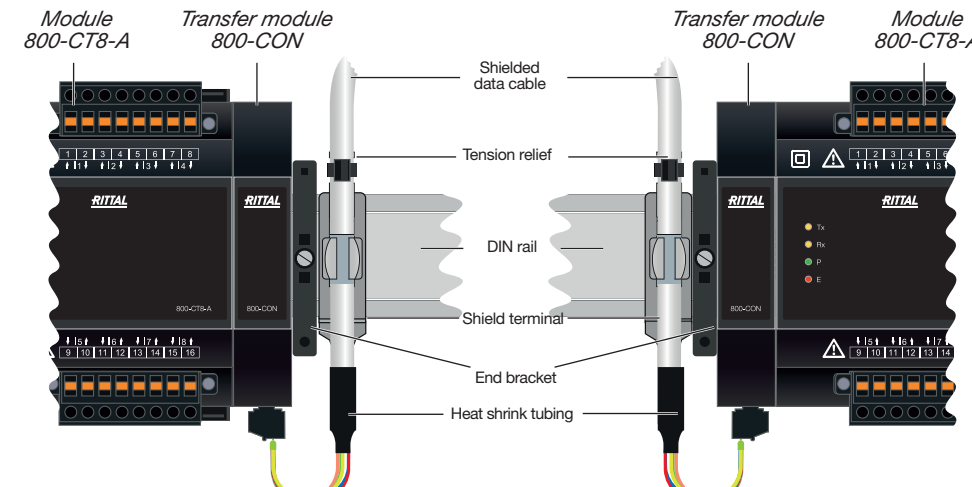
Fig. Example of "Device and module series": Wiring of the transfer module (output)
