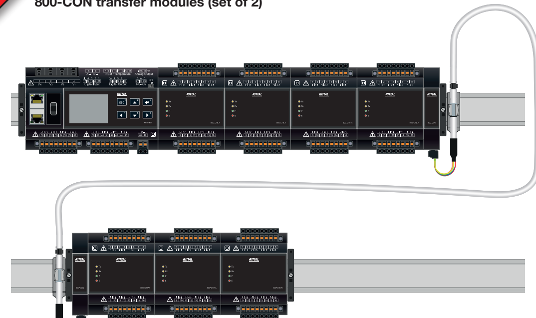
Example of a measuring device and module topology.
