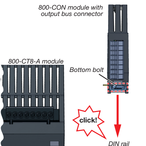
Example: Mounting of the 800-CON transfer module with output bus connector
