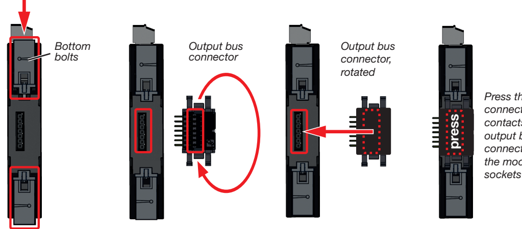
Fig.: Module 800-CON - rear view (with output bus connector)
