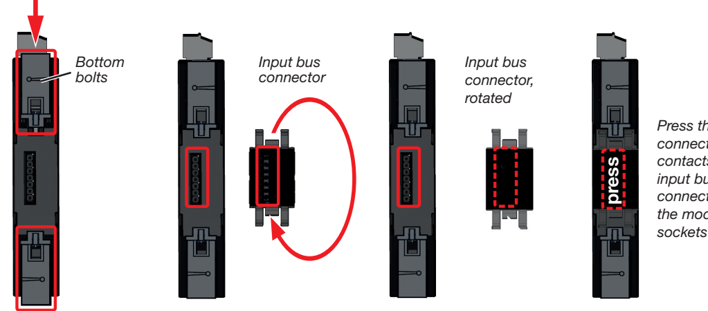
Fig.: Module 800-CON - rear view (with input bus connector)
