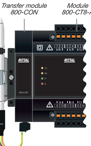
Fig. Example "Remote module series": Wiring of the transfer module (input)
