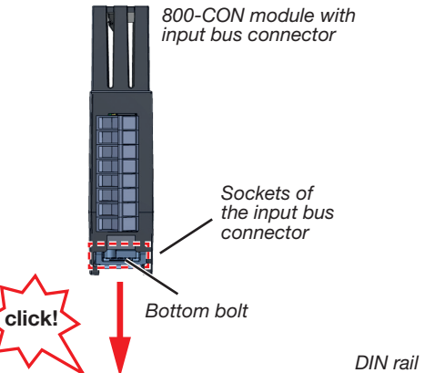
Example: Mounting of the 800-CON transfer module with input bus connector of the remote measuring point
