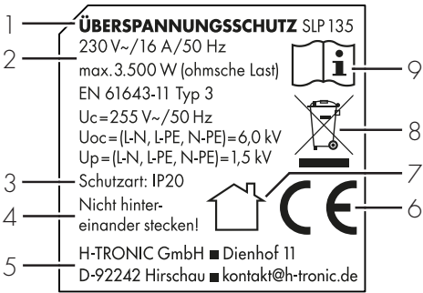
Figure 1 Nameplate
