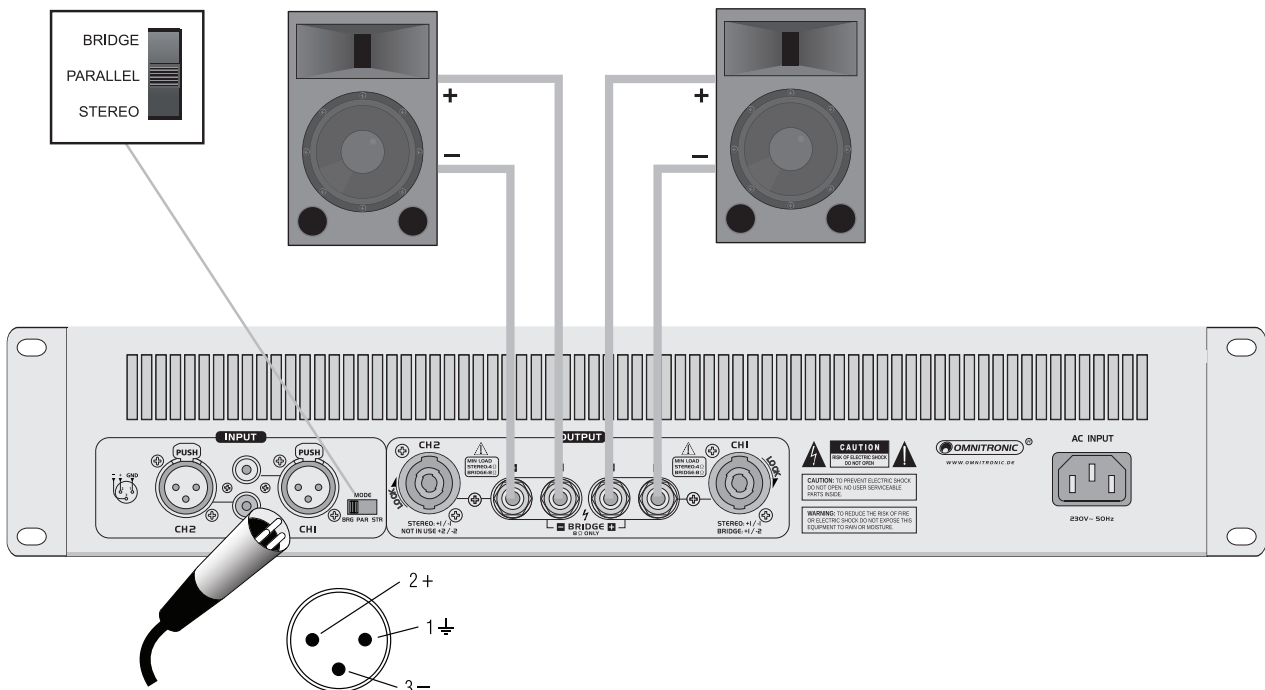
Fig. 6 Bridge wiring using the screw terminals
