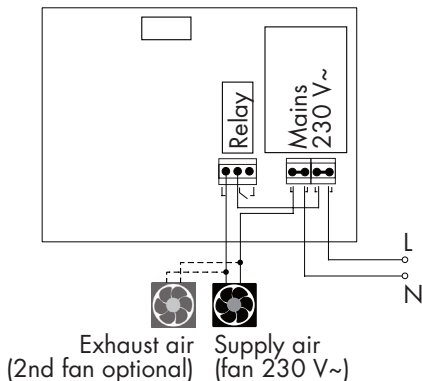
Figure 23 Application example for cellar drying
