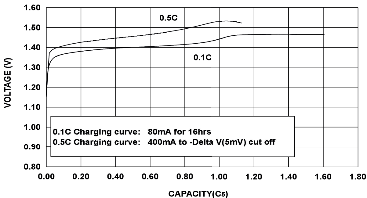
CHARGING CURVE OF BPI-50AA800 CELL
