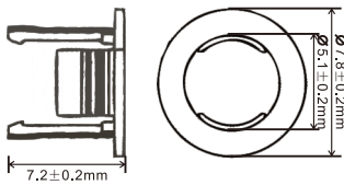
Indicator holder
