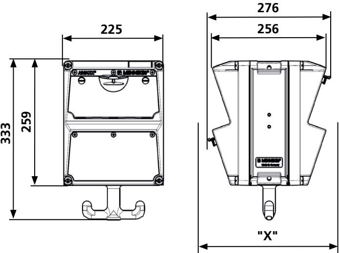
Dimension "X" with installed sockets (sockets are not shown in this diagram)
