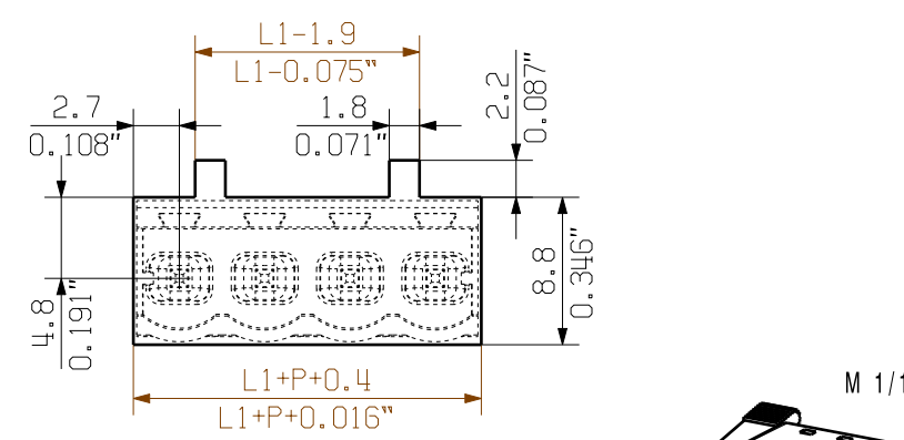
MIN. FRONT PLATE CUT-OUT
