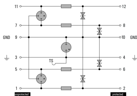
Complete module, indirect earthing
