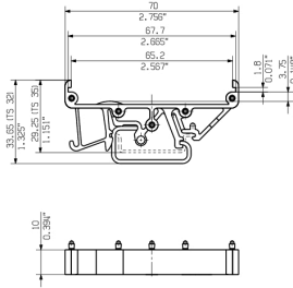
LOCKING-FOOT MIDDLE
