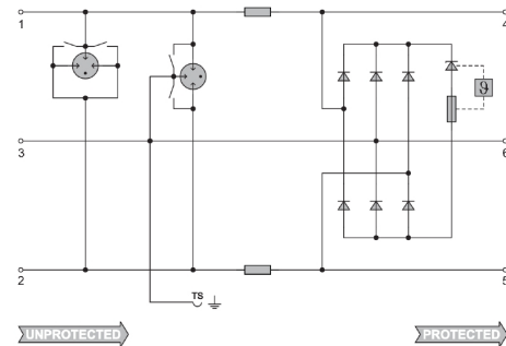
Circuit diagram
