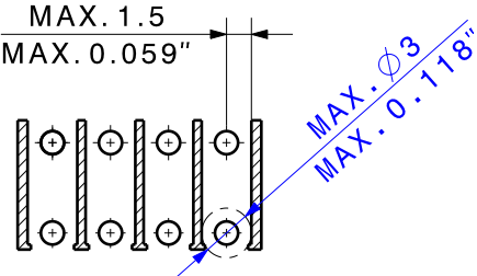
PASTE-FREE AREA
