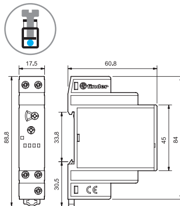
80.41 Morsetti a vite
