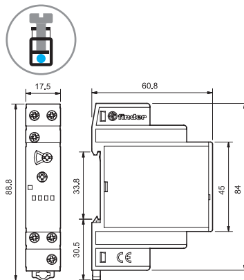
80.71 Morsetti a vite
