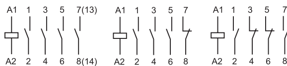
4 NO (4310) 3 NO + 1 NC (4710) 2 NO + 2 NC (4610)
