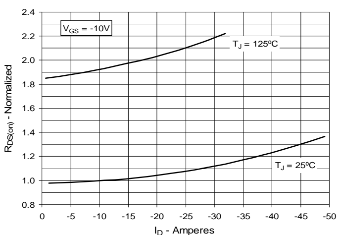
Fig. 5. R_{DS(on)} Normalized to I_D = -10A vs. Drain Current
