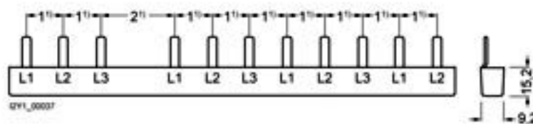
1) Pin spacings in MW (Modular widths, 1 MW = 18 mm).
